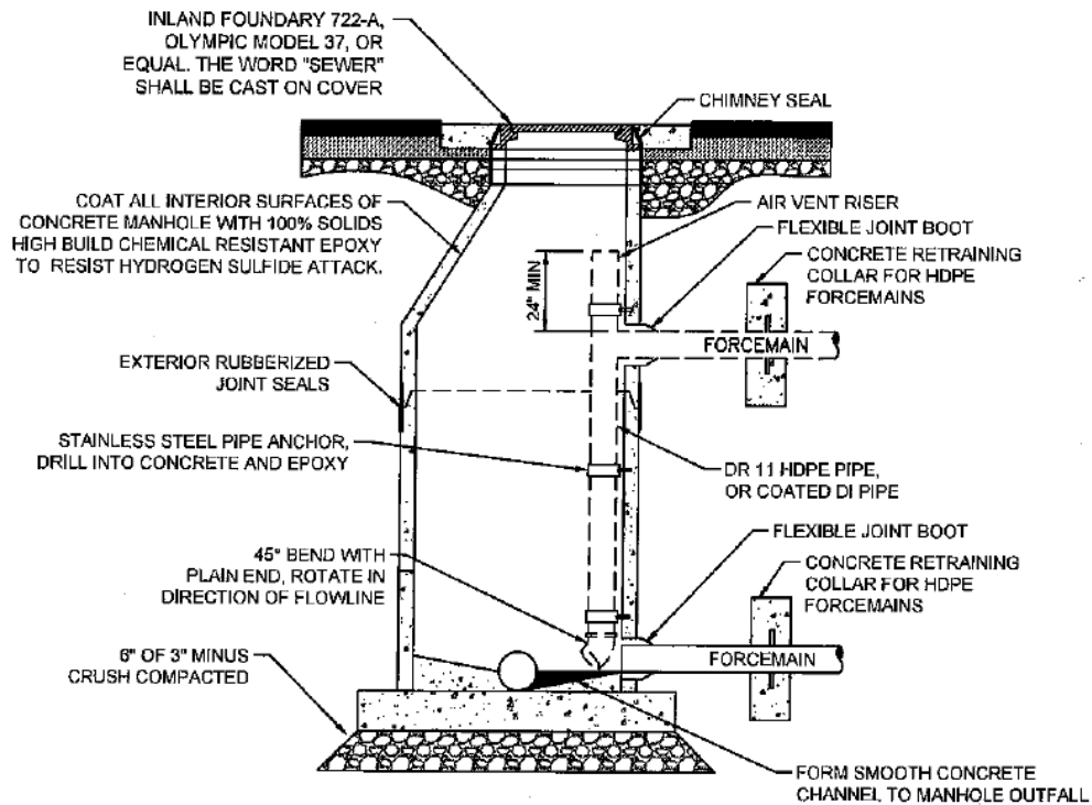
S-7 FORCEMAIN DISCHARGE MANHOLE DETAIL
