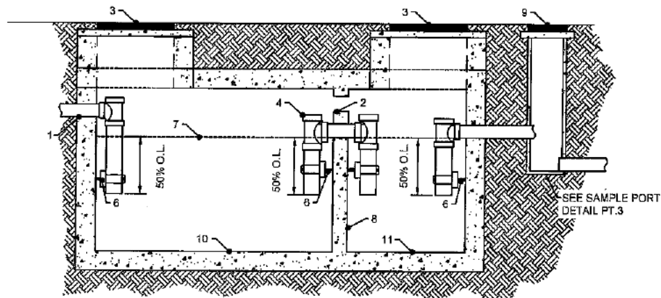
ELEVATION VIEW
