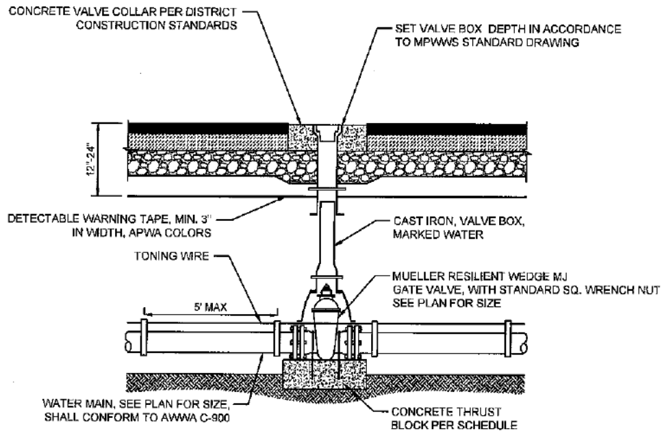
W-8 TYPICAL MJ GATE VALVE SECTION DETAIL
